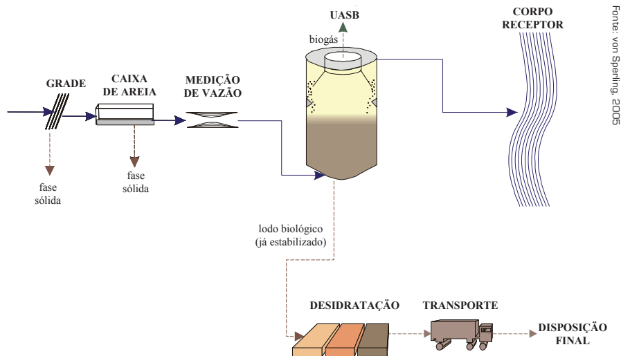
Reator UASB
